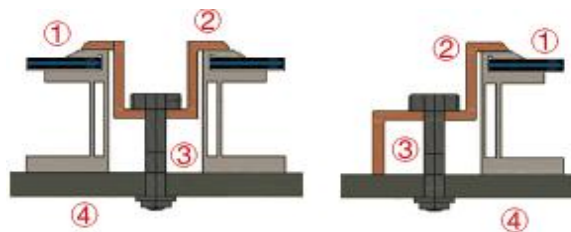
①frame ②Clip ③M8 bolt ④ mounting rail
